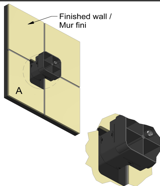
DETAIL A
